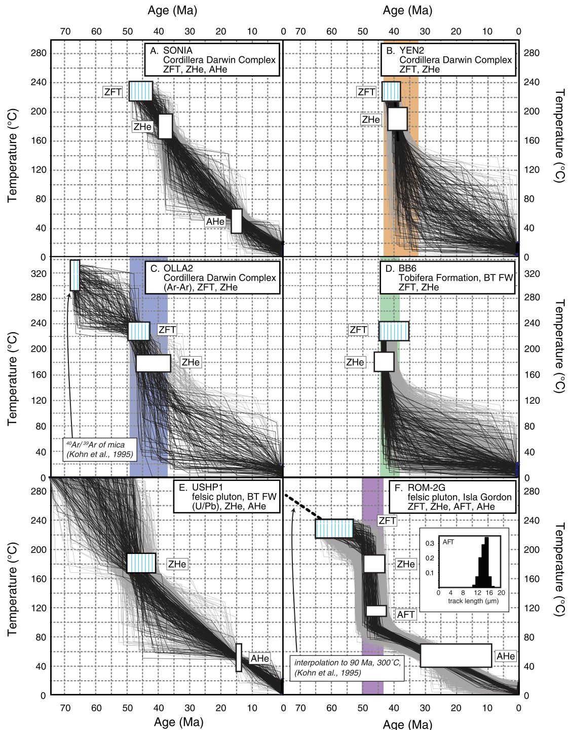
Fig. 3 Inverse models of T - t pathways for samples collected from the Fuegian Andes. White boxes with vertical blue dashed lines represent a priori constraints from ZFT or ^{40}\text{Ar}/^{39}\text{Ar} data which the T - t paths were forced through. The white boxes represent approximate locations of other thermochronometers for which individual closure temperatures were calculated during each model iteration. Black lines reveal model pathways with goodness-of-fit (GOF: Ehlers et al. , 2005) > 0.5 , while those in grey have GOF of < 0.5 but > 0.05 . Coloured boxes bracket periods of maximum exhumation rates determined by eye from each model. All errors in the inverse model are at the 1\sigma level.
