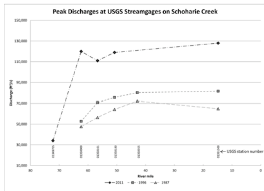
Figure 1: Peak discharges at U.S. Geological Survey streamgages on Schoharie Creek during floods of 1987, 1996 and 2011.
