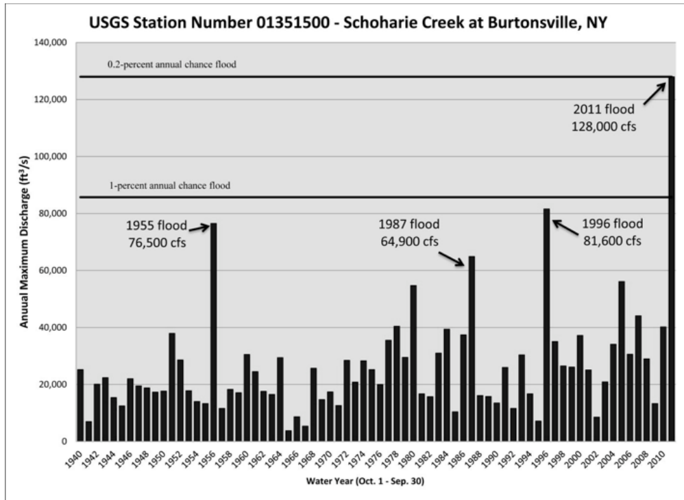
Figure 4: Annual peak discharges for the period-of-record at USGS station number 01351500 – Schoharie Creek at Burtonsville, NY (0.2 and 1-percent annual chance of flood discharges from FEMA, 2012).
