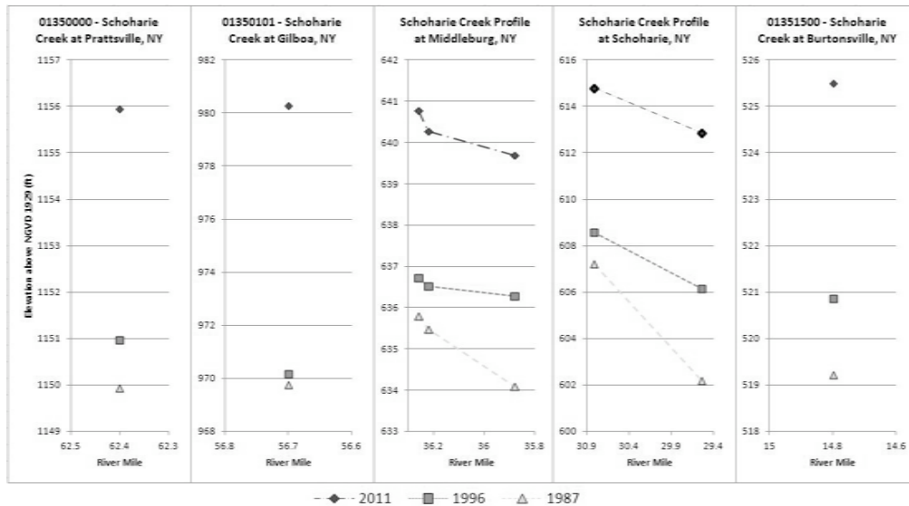
Figure 2: High-water mark elevations surveyed at selected U.S. Geological Survey streamgages and communities on Schoharie Creek following floods of 1987, 1996 and 2011.
