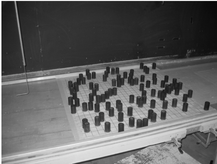
Figure 1: Experimental set-up of roughness elements utilizing a random array with 16.5% porosity.
