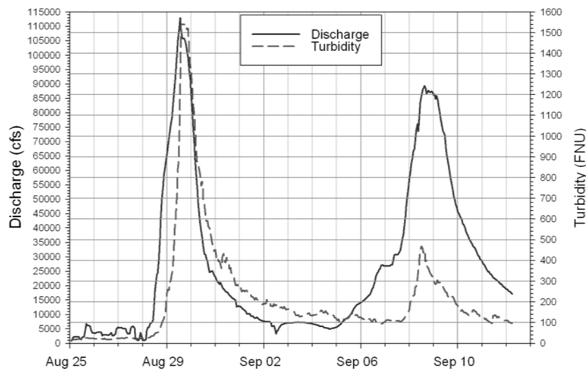
Figure 1: Hourly discharge and turbidity measured on the Mohawk River at Cohoes, NY during Irene and Lee in late summer 2011 (data from USGS).
