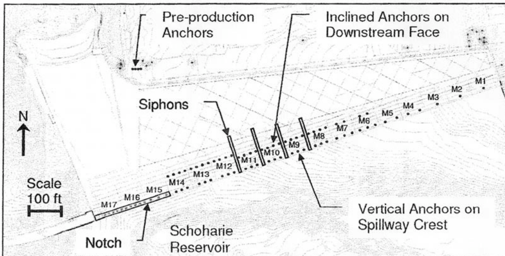
Figure 4 shows the placement of the anchors in the spillway (Zicko et al. 2007).
