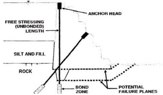
Figure 2 illustrates a typical anchor installation in the Gilboa Dam Spillway (Zicko et al. 2007).
