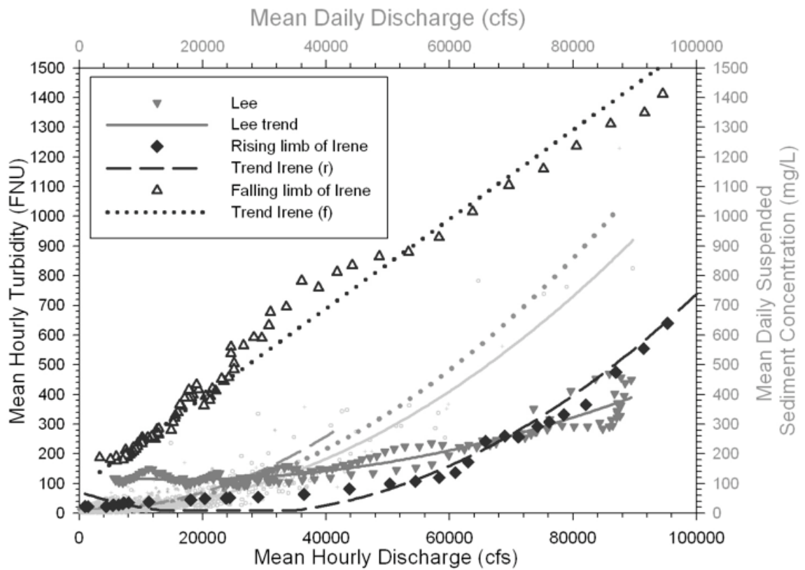
Figure 2: Mean hourly discharge and turbidity in the Mohawk River measured at Cohoes, NY during Irene and Lee. Light gray (background) points represent the daily values over the periods between 1954-57 and 2004-07.
