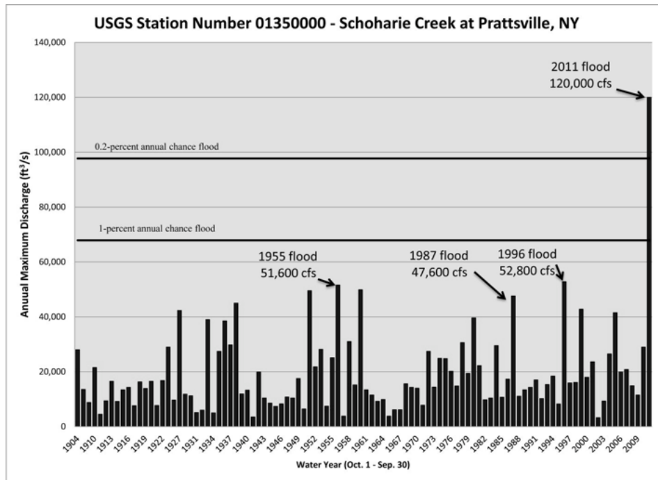
Figure 3: Annual peak discharges for the period-of-record at USGS station number 01350000 – Schoharie Creek at Prattsville, NY (0.2 and 1-percent annual chance of flood discharges from FEMA, 2008).
