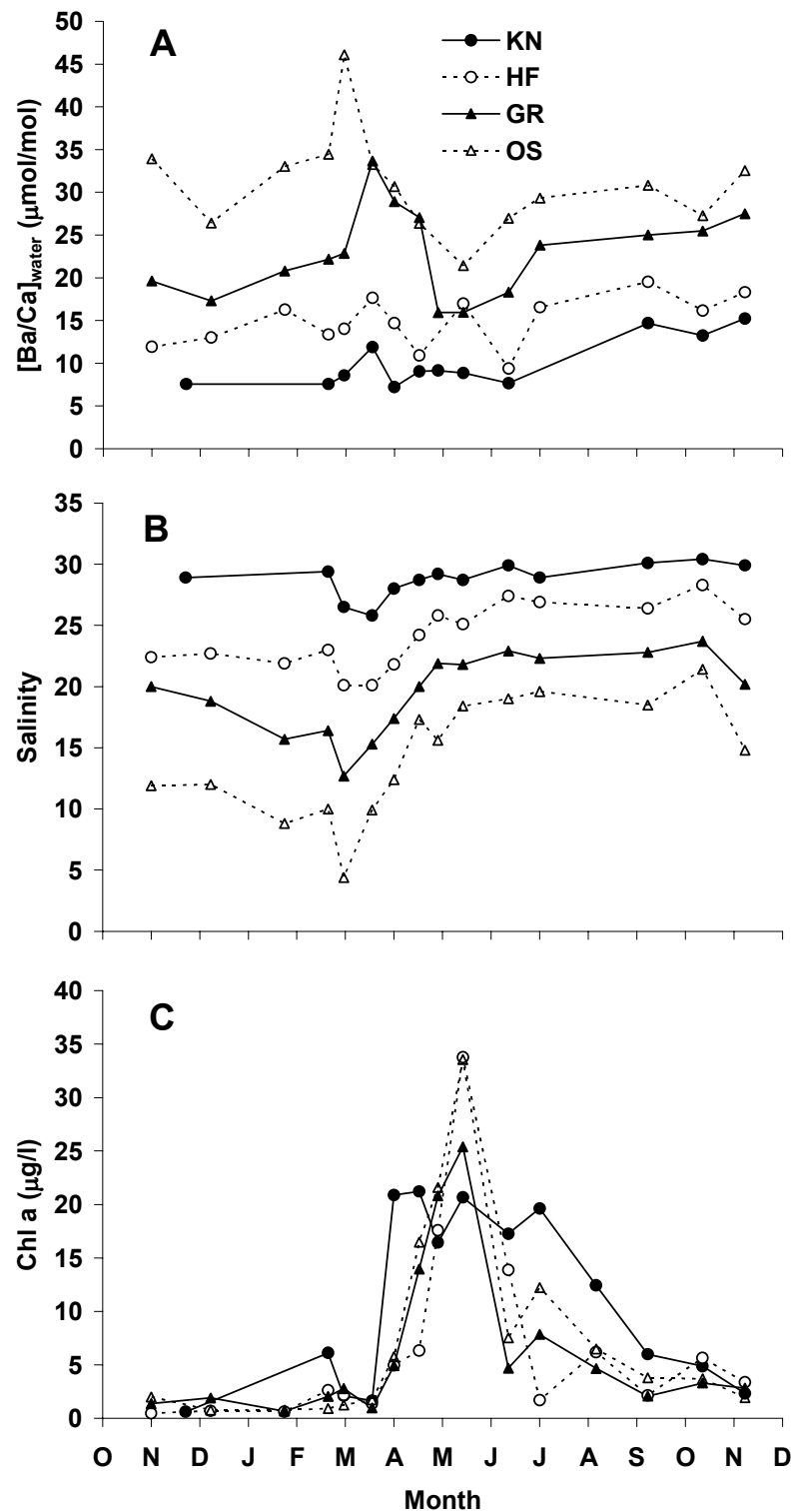
Figure 5. Dissolved [\text{Ba}/\text{Ca}]_{\text{water}} (A), salinity (B) and Chl a (C) at the four Schelde sites measured over one year (Nov. 2001 - Nov. 2002).
