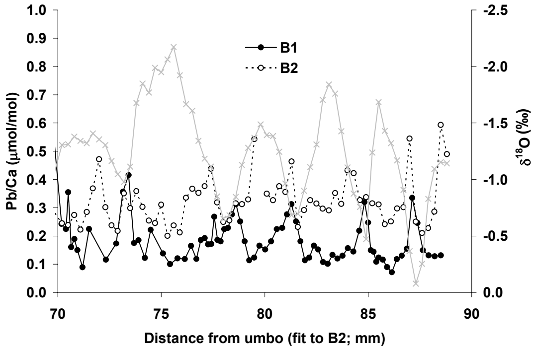
Figure 4. Pb/Ca data from the slow growing region of the Puget Sound (Washington, USA) shells. Data are the same as Figure 2D, but allow a detailed look at the variations in the profile.
