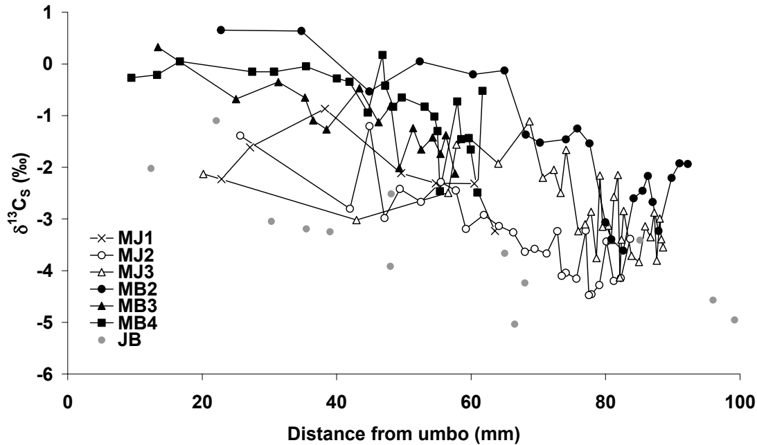
Figure 6. Annual shell \delta^{13}\text{C}_s from M. mercenaria shells collected at two sites (Johnson Creek, MJ shells and Back Sound, MB shells) plotted versus shell length. Data from JB shells are also given, but it should be noted that these samples represent less than one year and thus are expected to have a higher variability than the other shells which integrate a full year of growth.
