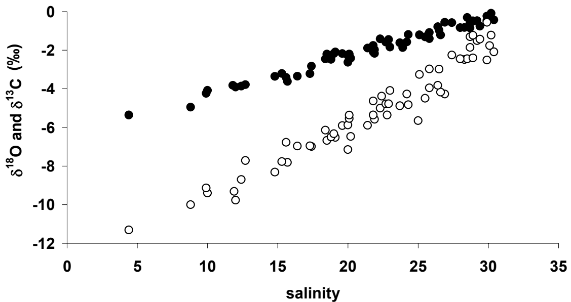
Figure 4. Relationship between salinity and \delta^{18}\text{O}_W (filled symbols) and \delta^{13}\text{C}_W (open symbols) in Schelde waters (see Chapter 10 for sampling locations) sampled at least monthly over a full year (data from Gillikin, unpublished). The simple linear regressions are \delta^{18}\text{O}_W = \text{Salinity} * 0.20 (\pm 0.01) - 6.31 (\pm 0.20) ( R^2 = 0.97 , p < 0.0001 , n = 63 ) and \delta^{13}\text{C}_W = \text{Salinity} * 0.39 (\pm 0.03) - 13.71 (\pm 0.57) ( R^2 = 0.94 , p < 0.0001 , n = 63 ).
