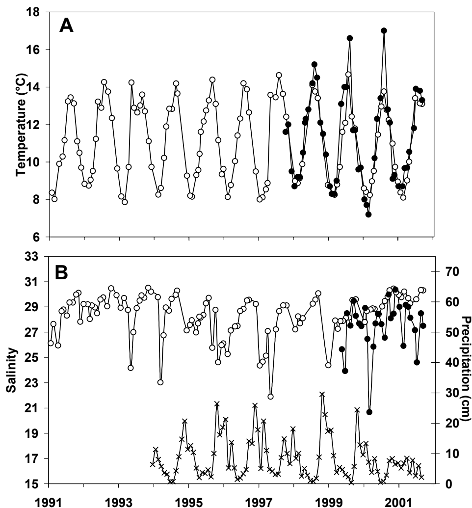
Figure 3. (a) Temperature records at both the shell collection site (Carkeek Park; solid circles) and at the offshore station (PSB003; open circles) and (b) salinity data from both stations (symbols as in a) as well as monthly average precipitation data from Seattle, Washington (crosses).
