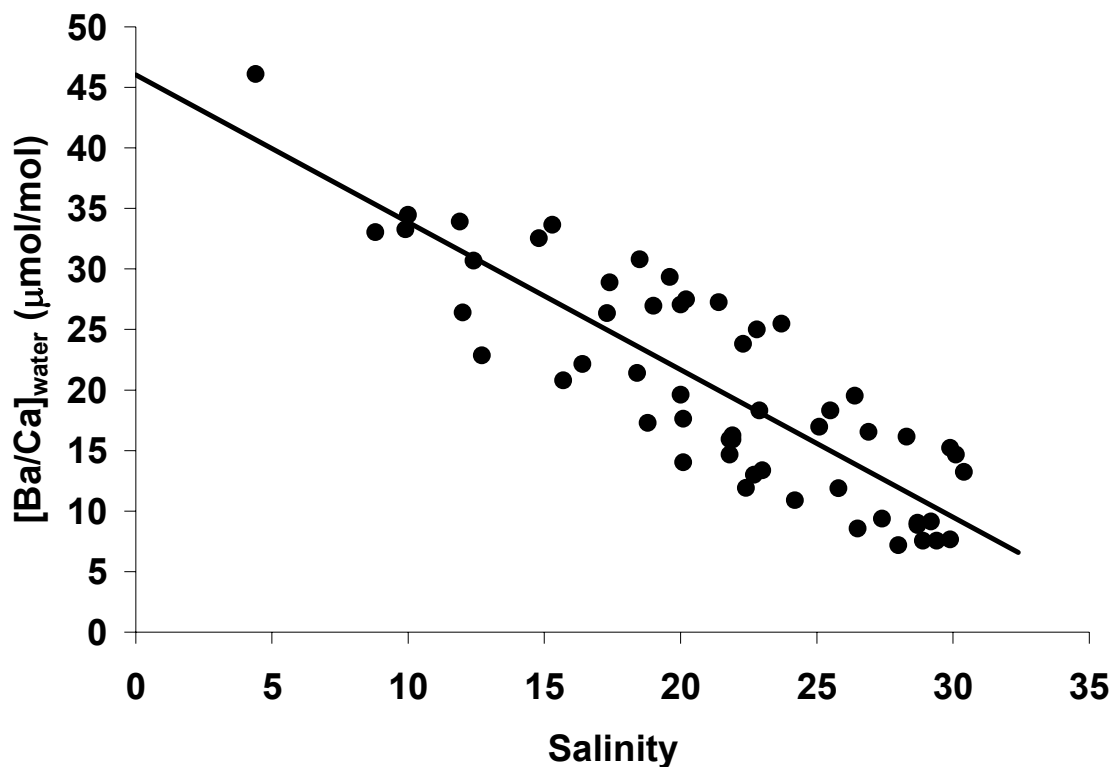
Figure 6. Salinity versus [\text{Ba}/\text{Ca}]_{\text{water}} including data from all sites and sampling dates. The linear relationship ( R^2 = 0.73 , n = 55 , p < 0.0001 ) is [\text{Ba}/\text{Ca}]_{\text{water}} = -1.22 (\pm 0.21) * \text{Salinity} + 46.05 (\pm 4.57) .
