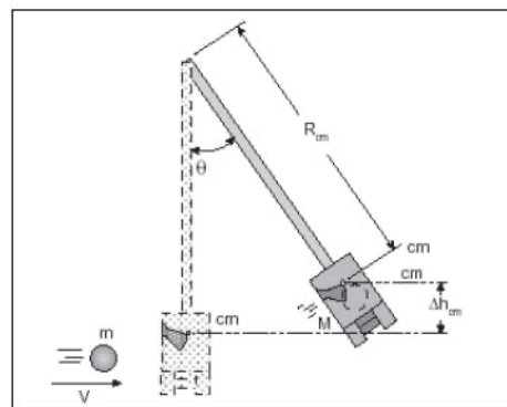
Figure 2: Figure 2: A ball of mass, m , and speed, v , is caught by the pendulum, which swings up to an angle \theta . https://www.pasco.com/products/lab-apparatus/mechanics/projectiles/ballistic-pendulum
