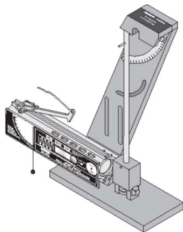
Figure 1: The ballistic pendulum apparatus. https://www.pasco.com/products/lab-apparatus/mechanics/projectiles/ballistic-pendulum
