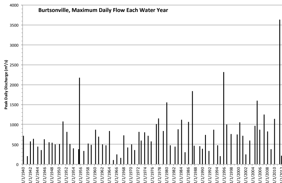
Figure 2: Maximum daily flow each year on Schoharie Creek at the Burtonsville gaging station. The lower part of the Schoharie Creek (Burtonsville) has had higher maximums since the 1970s.
